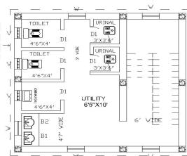
GIRLS TOILET FIRST FLOOR PLAN
