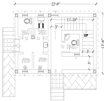
BOYS TOILET GROUND FLOOR PLAN
