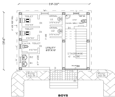
BOYS TOILET GROUND FLOOR PLAN
