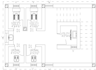
GIRLS TOILET FIRST FLOOR PLAN
